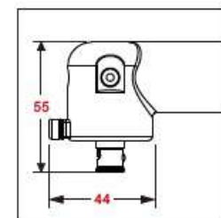
OP-311LHA F Rear exhaust 後排氣
