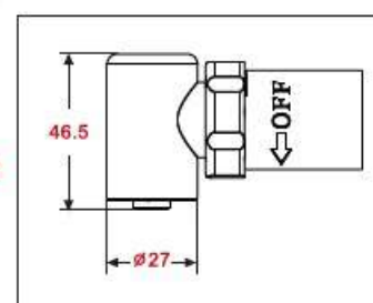
OP-304L90 F Rear exhaust 後排氣
