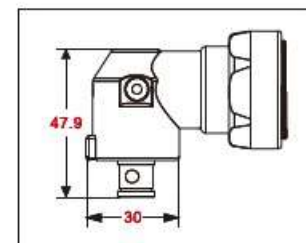
OP-301L90 F Rear exhaust 後排氣
