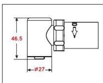
OP-302L90 F Side exhaust 側排氣
