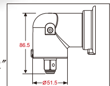
OP-130LH4 1/2" Side exhaust 側排氣
